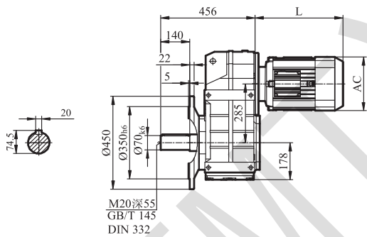
GFF97
