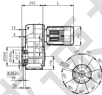
GFAF/GFHF/GFVF97
