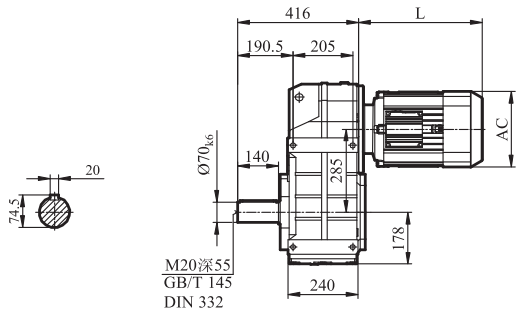
GF97
